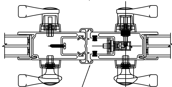
4 PANEL DOOR DETAIL
