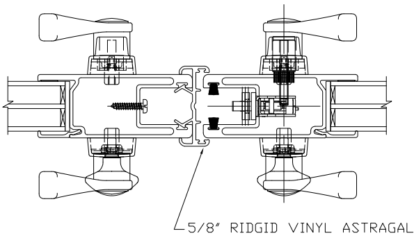
4 PANEL DOOR DETAIL
