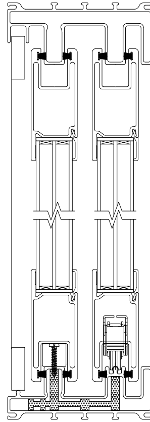
VERTICAL SECTION
