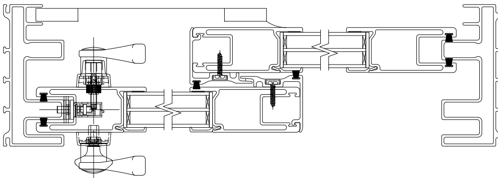
HORIZONTAL SECTION
