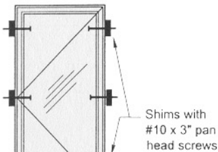
CASEMENT 300 SERIES
